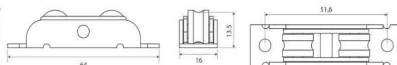
Product Drawing
