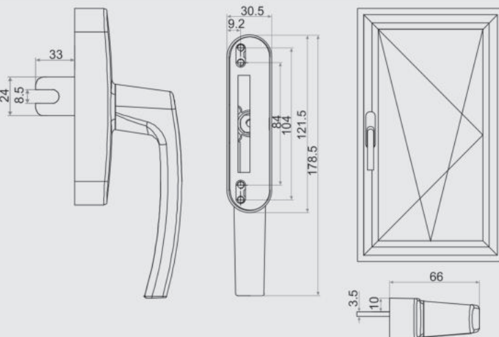
Product Drawing
