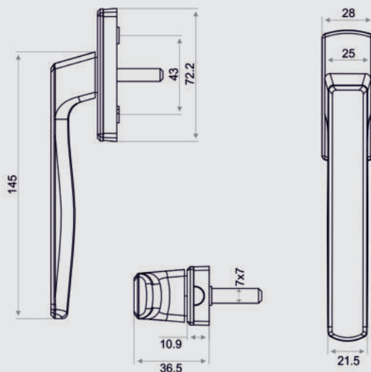
Product Drawing
