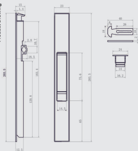
Product Drawing
