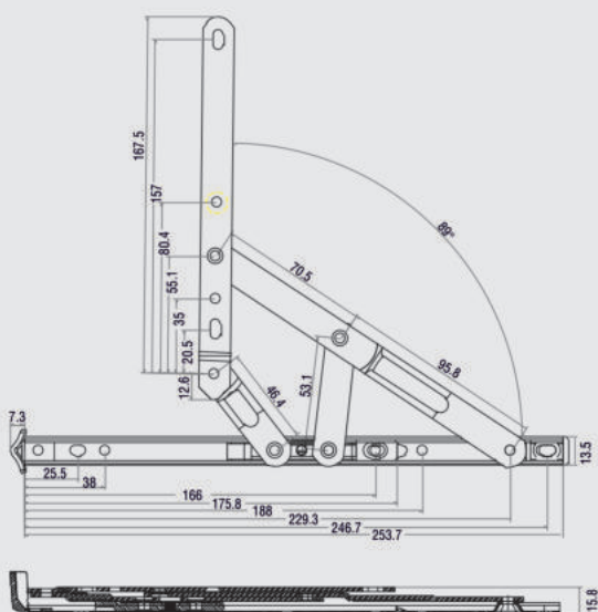
Product Drawing
