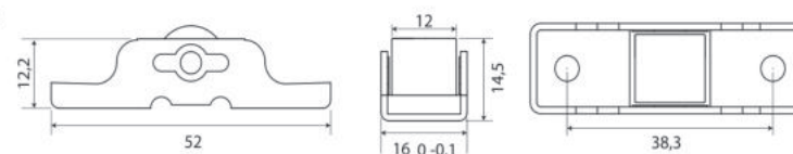
Description : Window Roller
