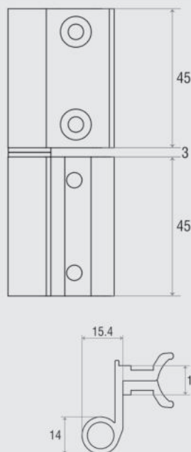
Product Drawing
