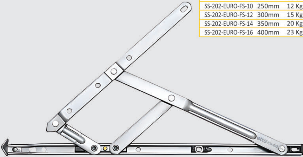
Product Drawing
