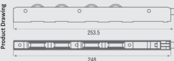
Description : Window Roller
