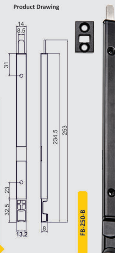
Product Drawing
