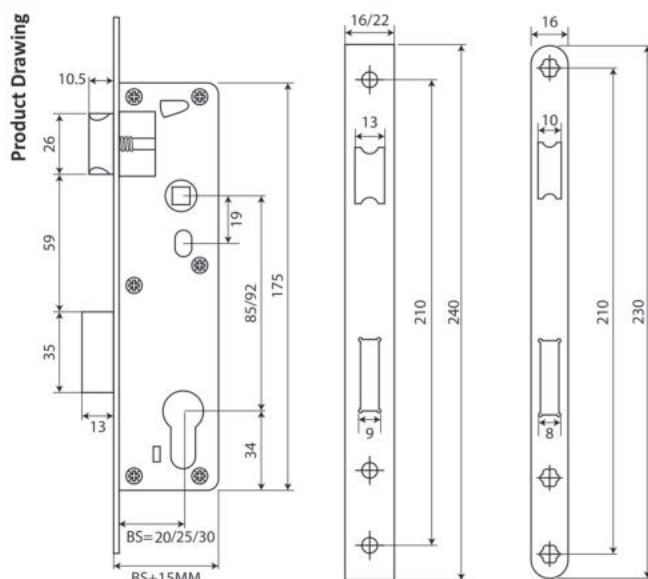
Description : Lock Body with Plate
