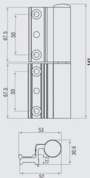
Product Drawing
