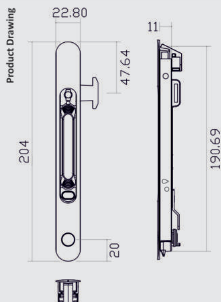
Description : Aluminium Conceal Lock (Key)
