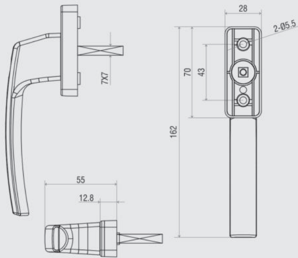
Product Drawing
