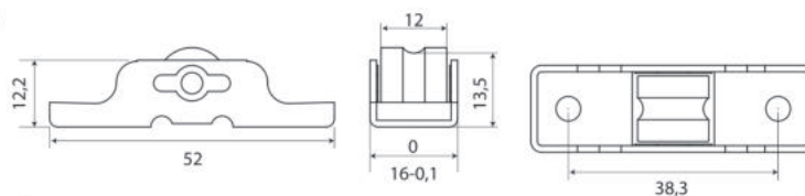
Description : Window Roller
