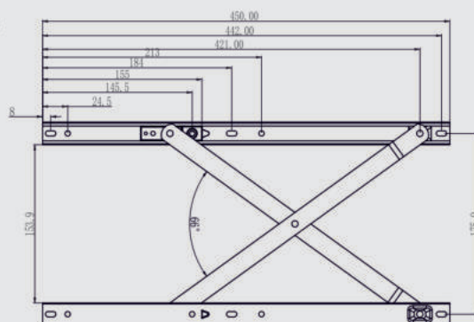
Product Drawing
