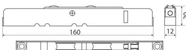
Description : Window Roller (Adjustable)
