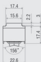
Description : Window Roller
