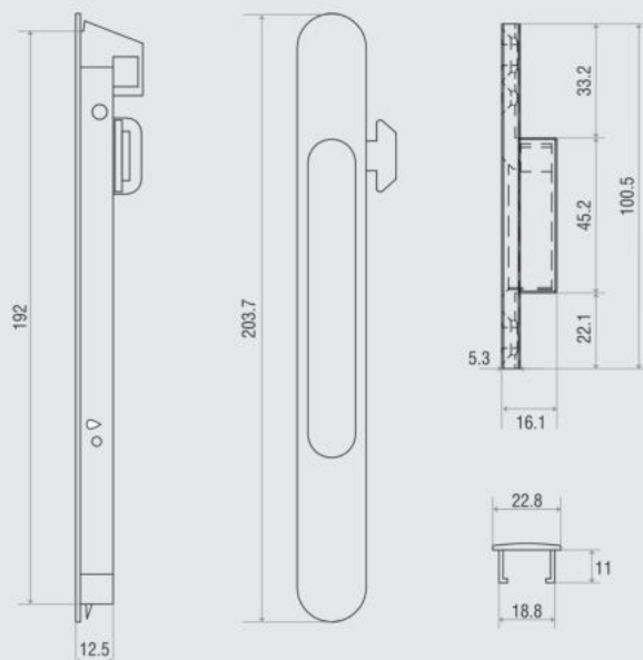
Description : Aluminium Conceal Lock
