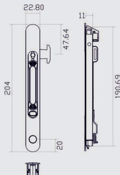
Product Drawing
