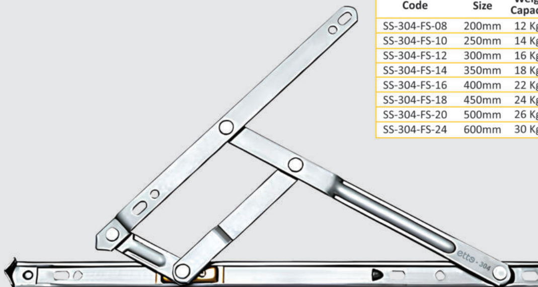
Product Drawing
