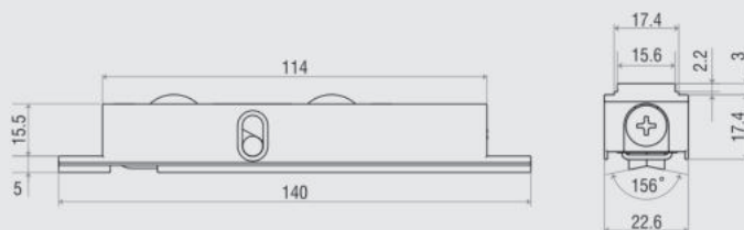
Description : Window Roller
