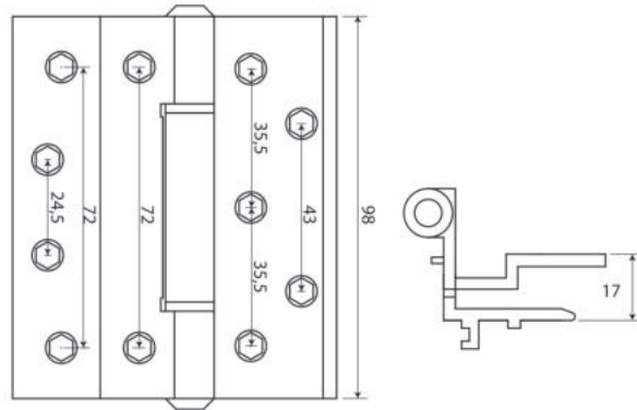
Product Drawing
