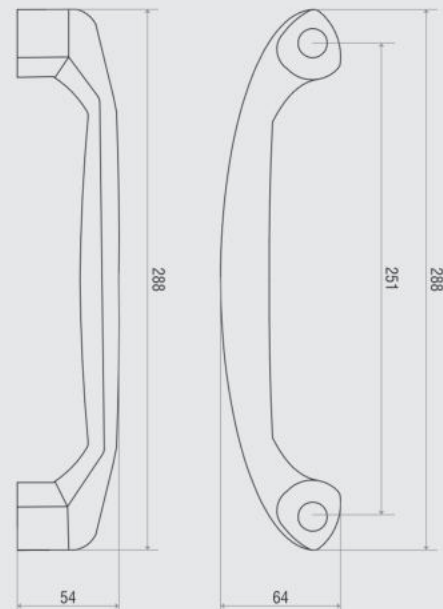
Product Drawing
