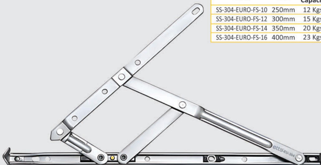
Product Drawing
