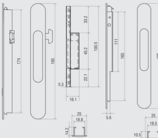
Product Drawing
