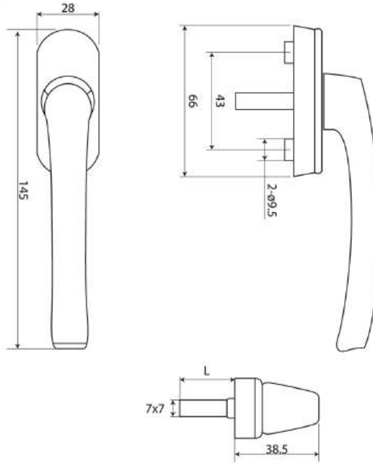
Product Drawing
