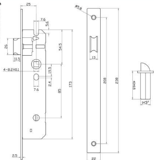
Product Drawing
