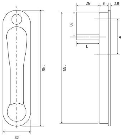
Product Drawing
