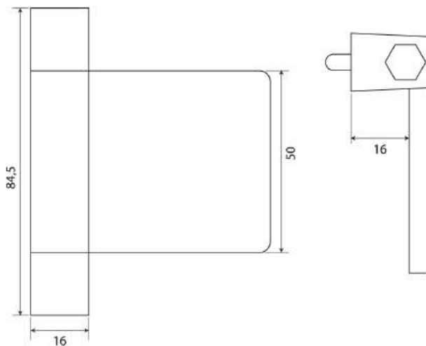
Product Drawing
