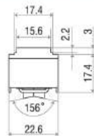
Product Drawing
