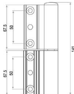
Product Drawing
