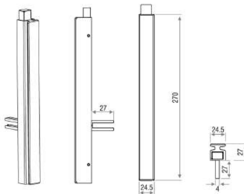
Product Drawing
