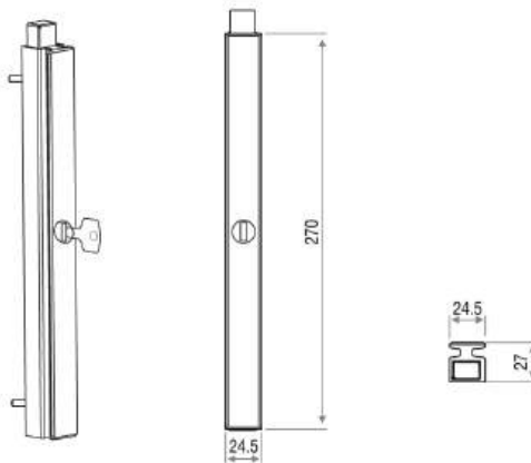
Product Drawing
