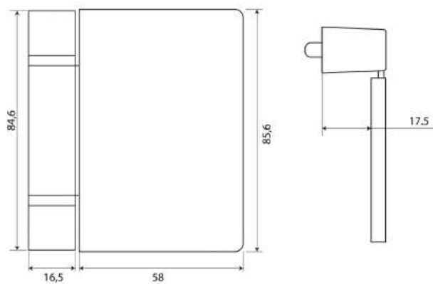
Product Drawing
