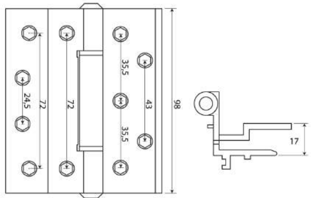
Product Drawing
